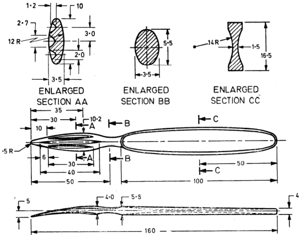
FIG. 1 KOCHER PATTERN DISSECTOR
